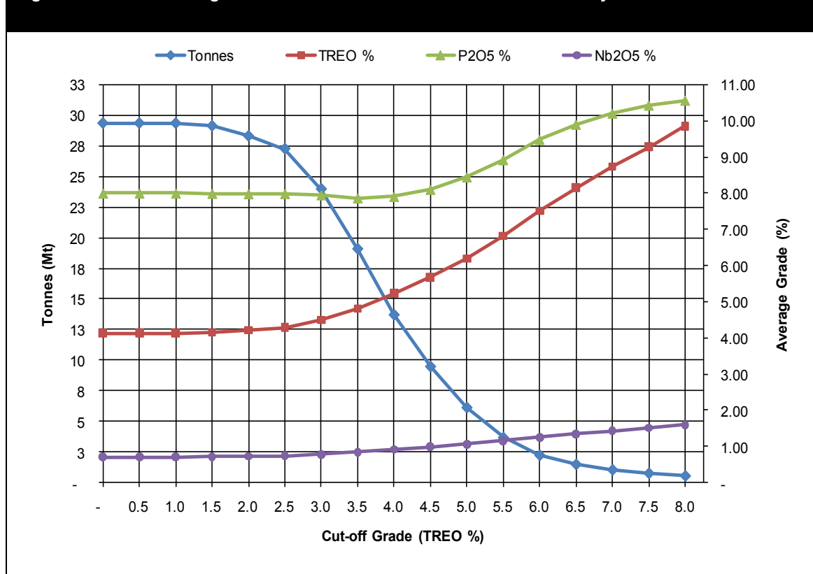
Figure 20 : Grade Tonnage Curve for REOs associated with the Araxá Project
