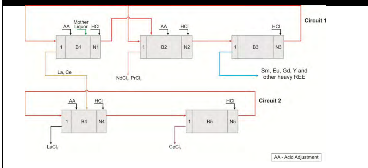
Figure 23: Solvent Extraction Route 2
